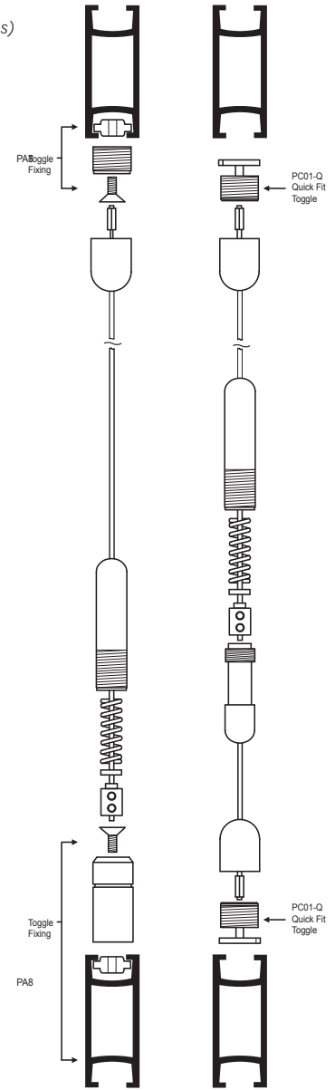
CA4 Cable Kit CQQ Cable Kit
